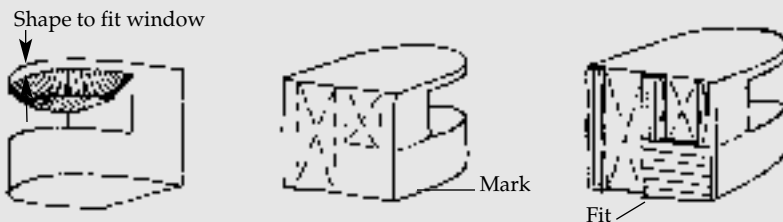
FIG. 13 – Beveling the Pilot House
